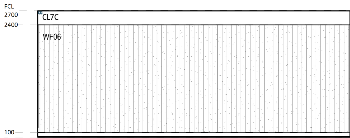
5 ELEVATION DETAIL 60-009 1 : 50
