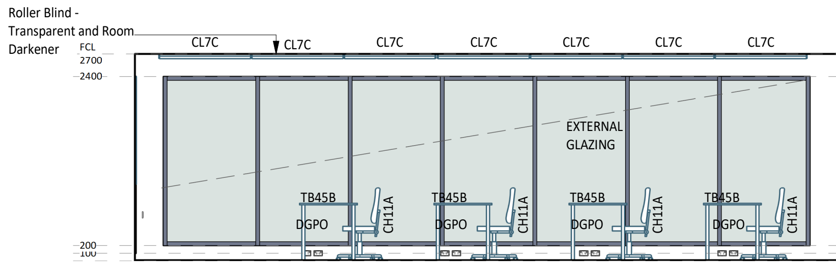
4 ELEVATION DETAIL 60-009 1 : 50
