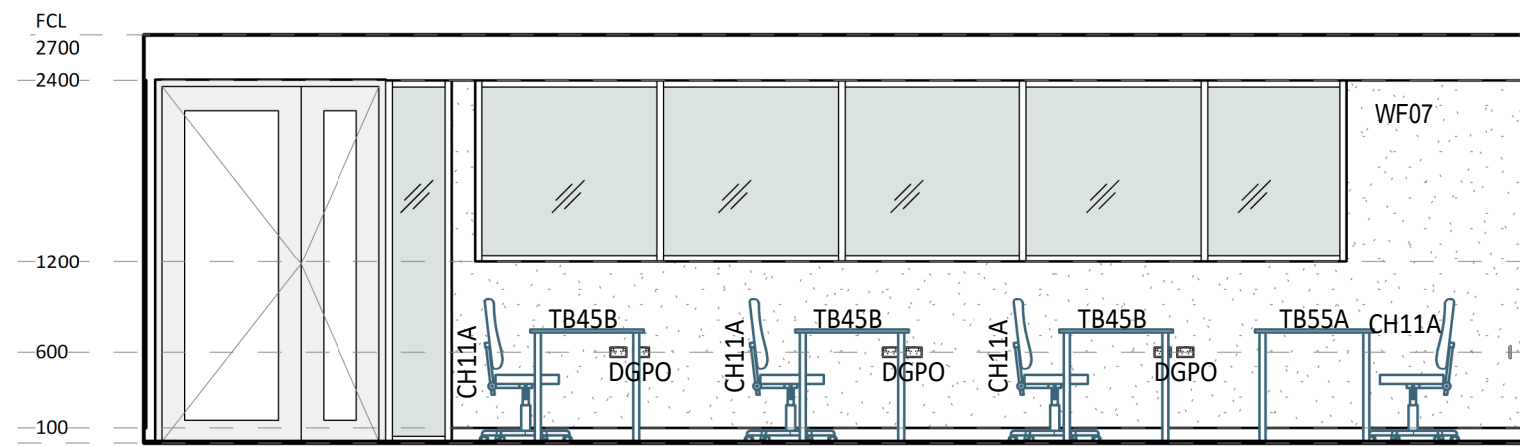
2 ELEVATION DETAIL 60-009 1 : 50
