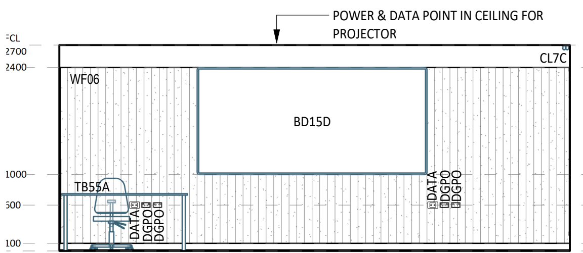
3 ELEVATION DETAIL 60-009 1 : 50
